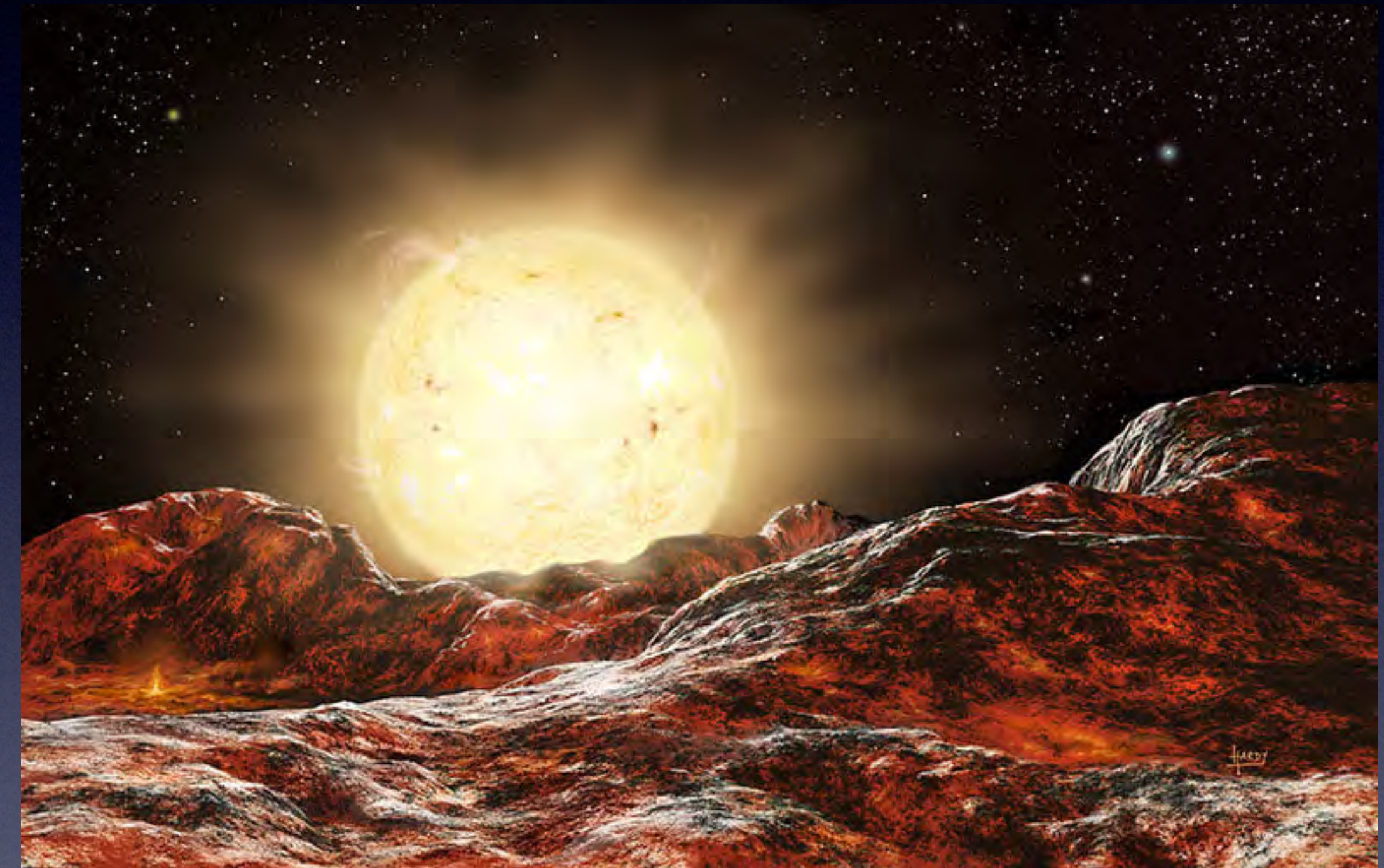
KEPLER 10B
